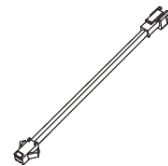
LN-SWCM-30 12"(300mm) LN-SWCM-60 24"(600mm) Type : Signal wire connect between modules
