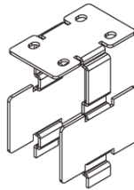
LN1-LA-ER Type: Light Leak-proof aluminum extrusion reinforce plate
